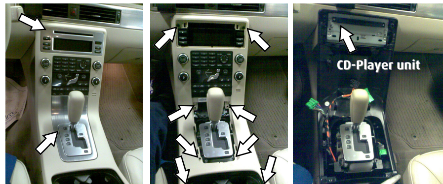
Pictures of center console removal in Volvo V70
